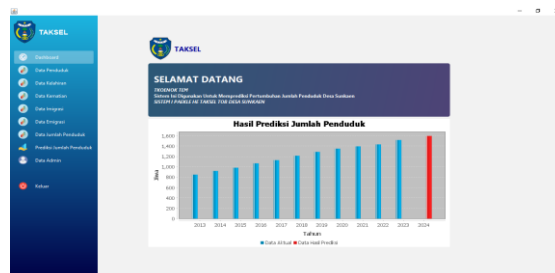
Gambar 6. Menu Dashboard
