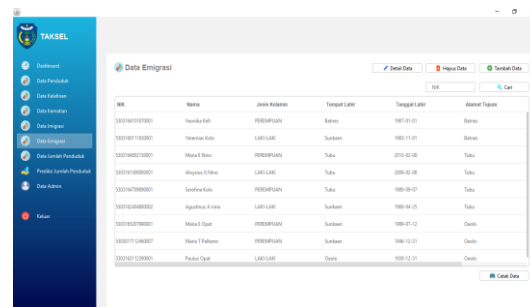
Gambar 11. Menu Emigrasi
